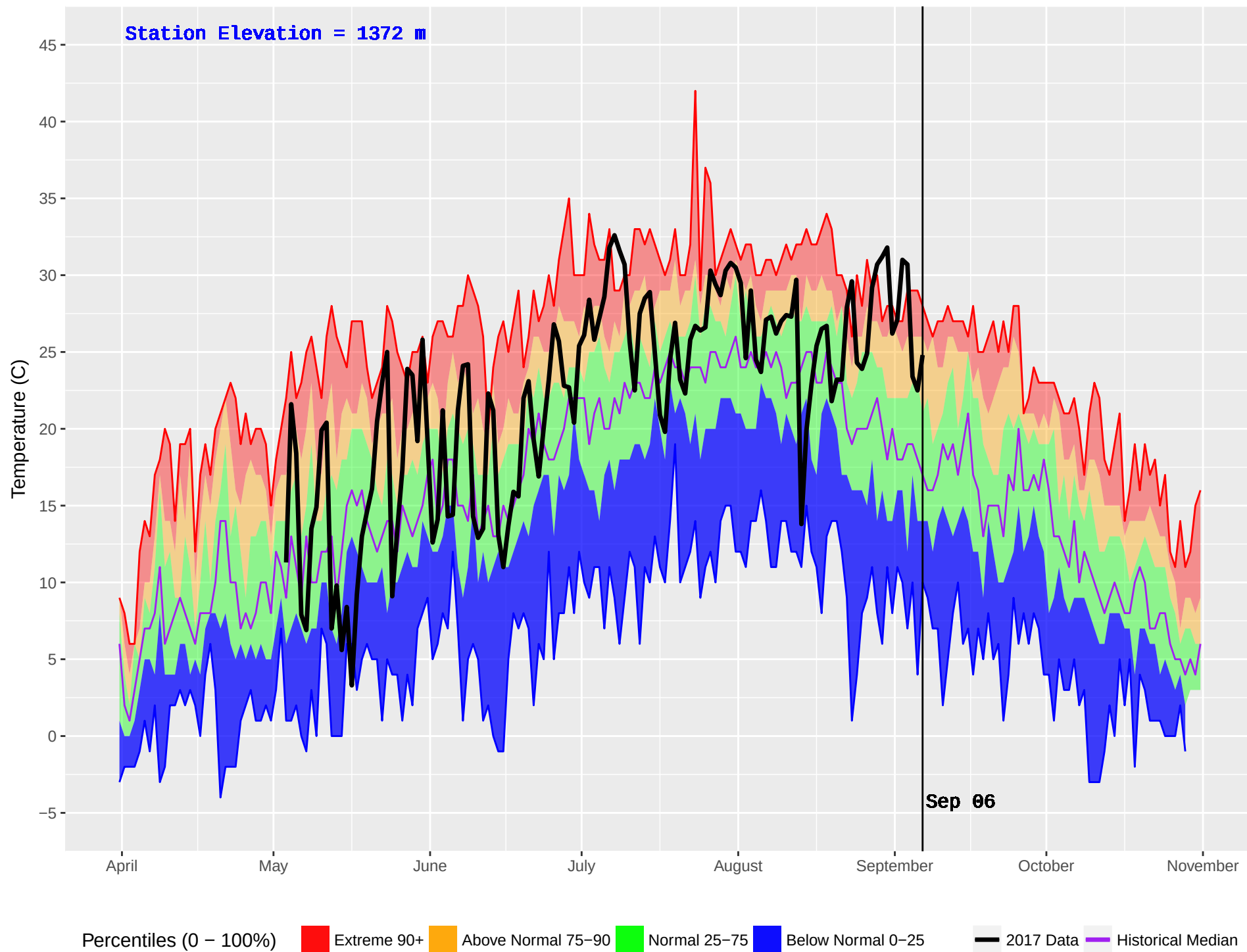
CHERRY LAKE (791) : Historical (1989–2016) and Current (2017) Noon Temperature
