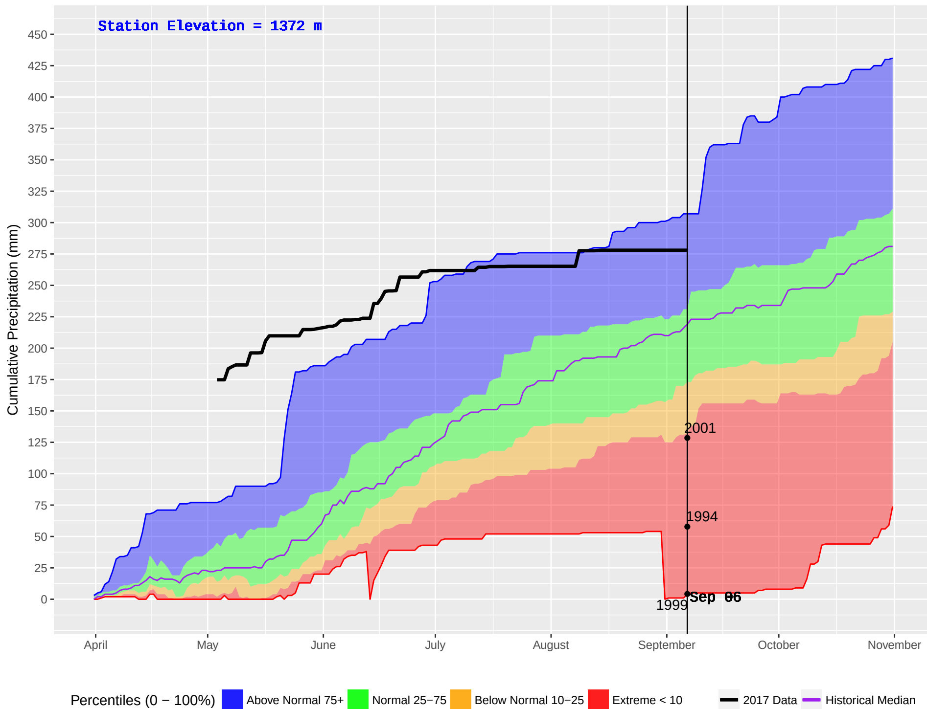
CHERRY LAKE (791) : Historical (1989–2016) and Current (2017) Noon Cumulative Precipitation
